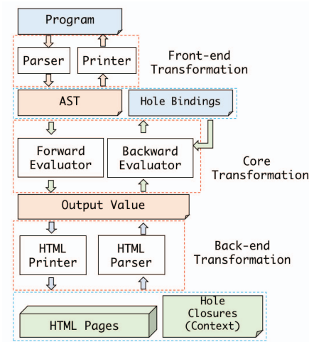
Figure 6: System Framework
